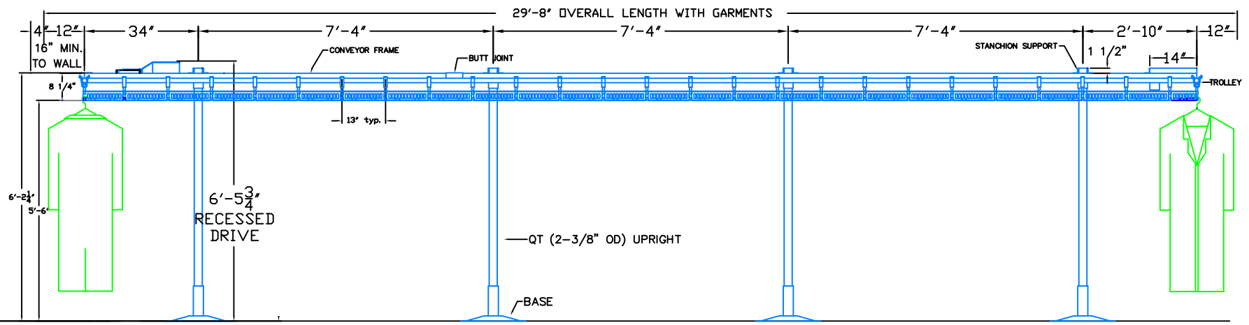
SIDE ELEVATION OF SYS 722-636
