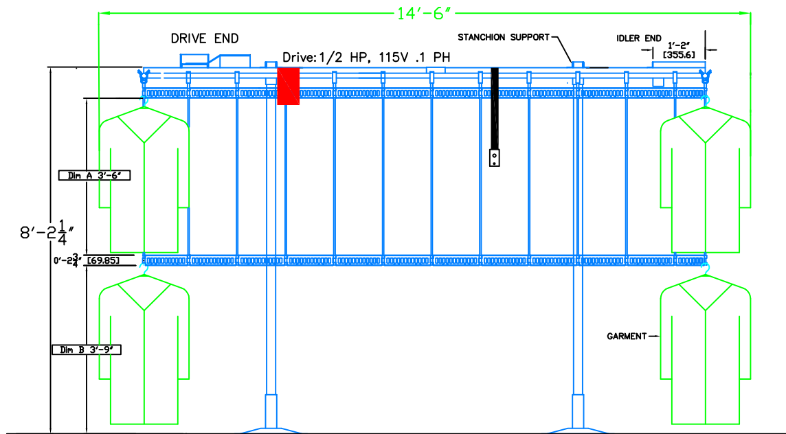
SIDE ELEVATION OF SYS 742-600
