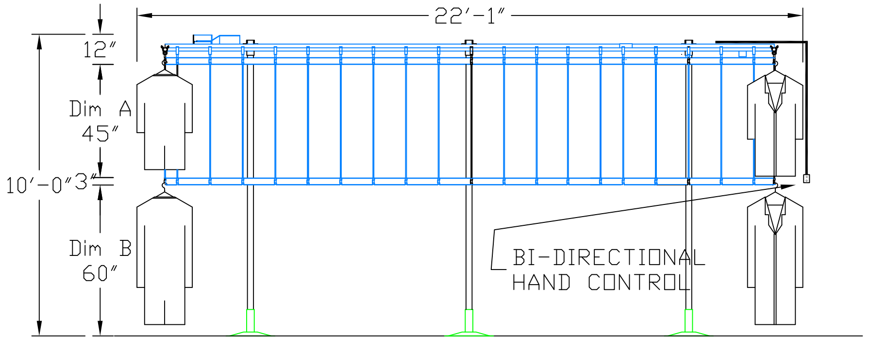
SIDE ELEVATION OF SYS 742-936
