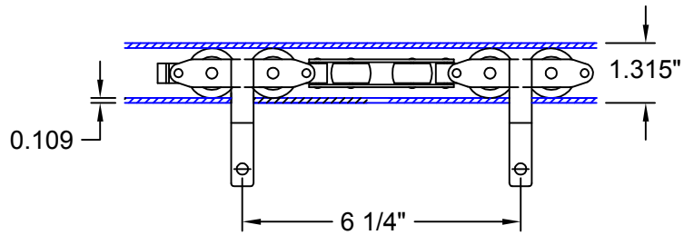
Detail A Chain detail
