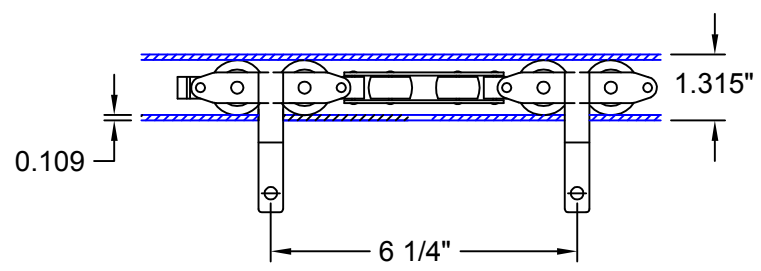
Detail A Chain detail
