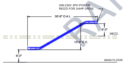
ELEVATION SHOWING SYS 211 TROLLEY BOOSTER (SYS 211-13-0-3)
