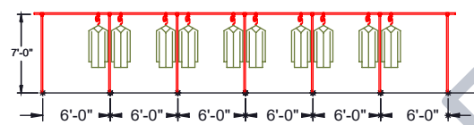
ELEVATION D-D 1/8" = 1'-0"
