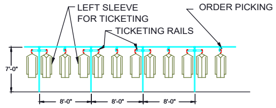
ELEVATION C-C 1/8" = 1'-0"
