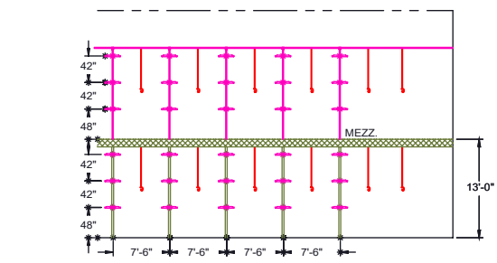
ELEVATION B-B 1/8" = 1'-0"
