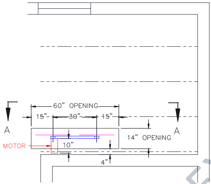
PLAN FLOOR OPENING REQUIRED: 14" X 60" 1/2" = 1'-0"
