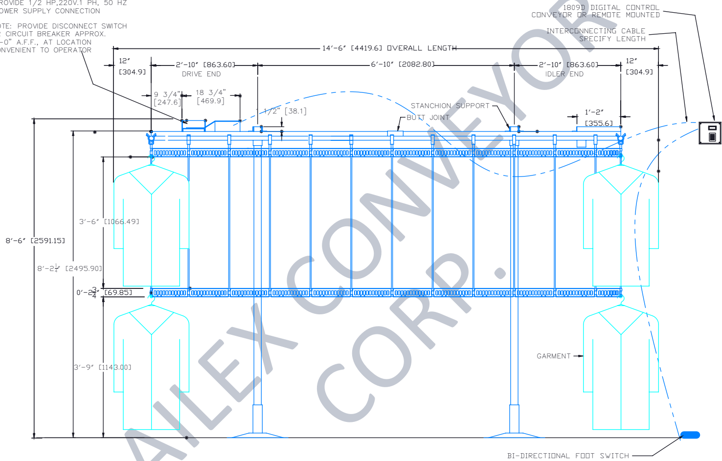
SIDE ELEVATION OF SYS 742-600
