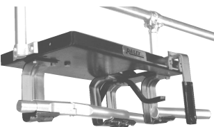
Master Switch - 2MS2 (2 way)
